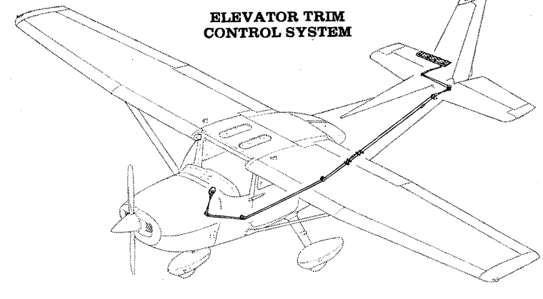
Figure 7-1. Flight Control and Trim Systems (Sheet 2 of 2)
