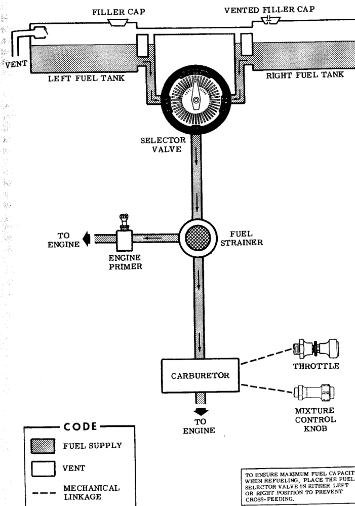
Figure 7-6. Fuel System (Standard and Long Range)
