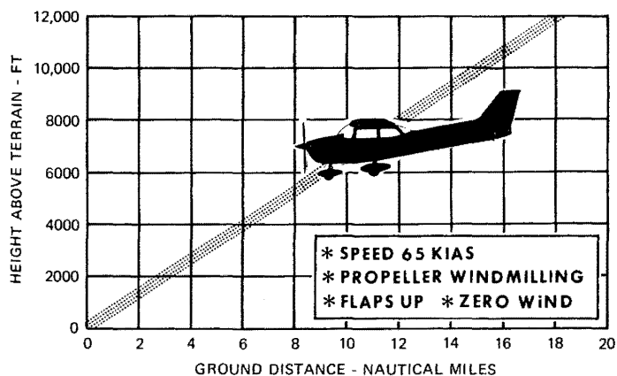
Figure 3-1. Maximum Glide
