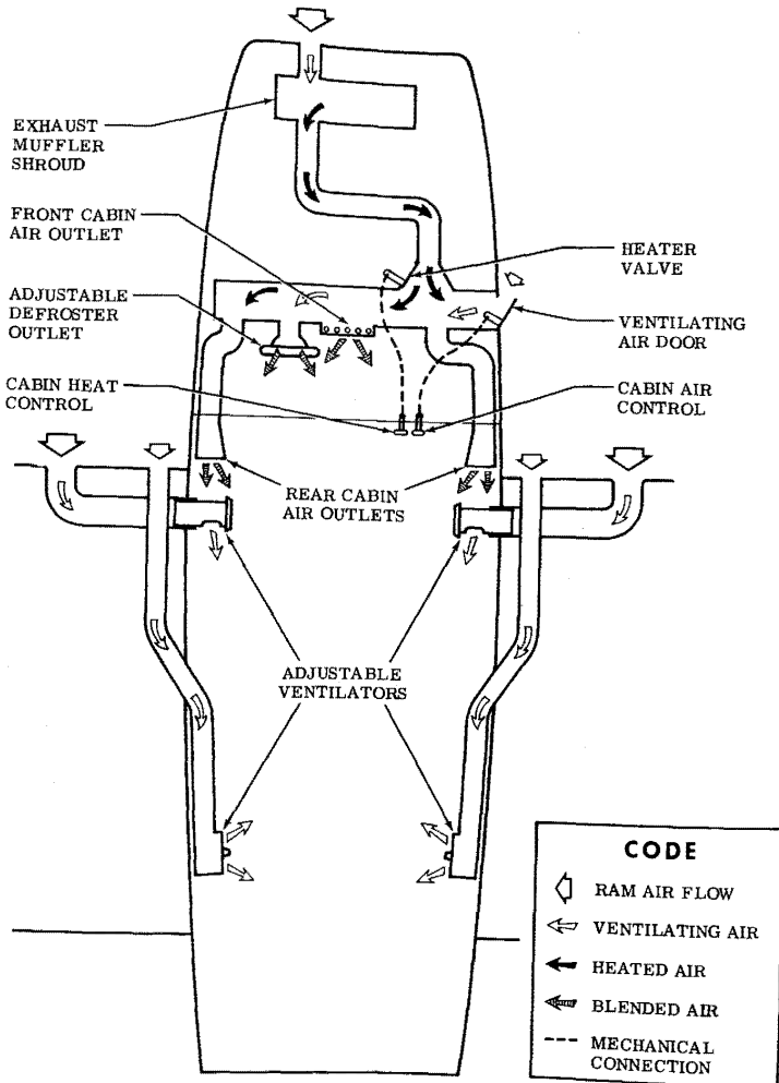
Figure 7-8. Cabin Heating, Ventilating, and Defrosting System
