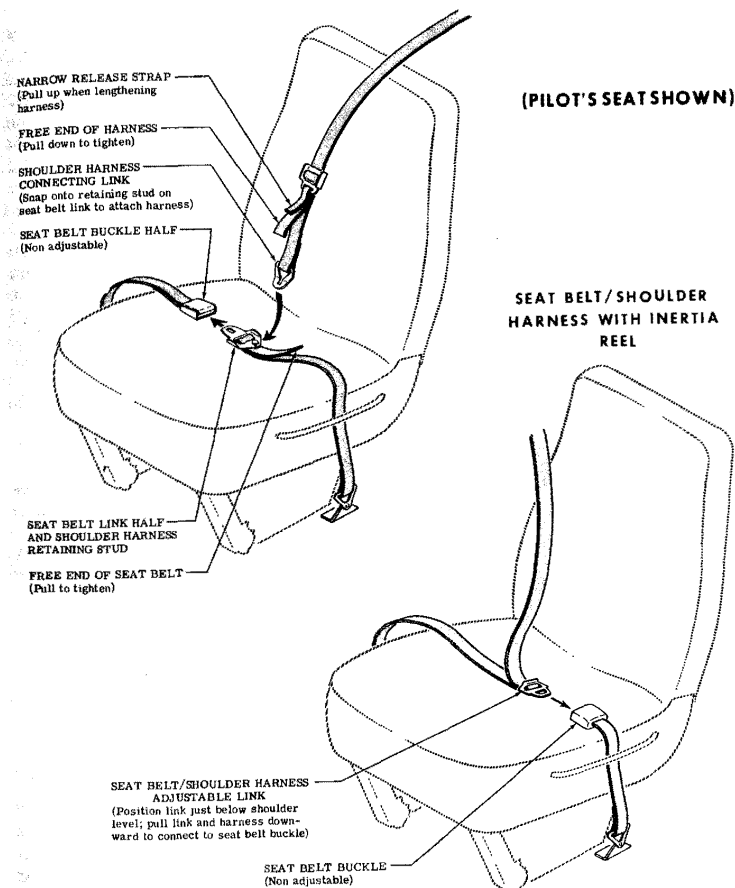
Figure 7-4. Seat Belts and Shoulder Harnesses
