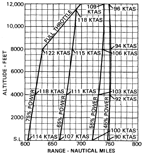
Figure 5-8. Range Profile (Sheet 2 of 2)
