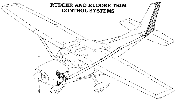
Figure 7-1. Flight Control and Trim Systems (Sheet 1 of 2)
