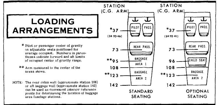
Figure 6-3. Loading Arrangements
