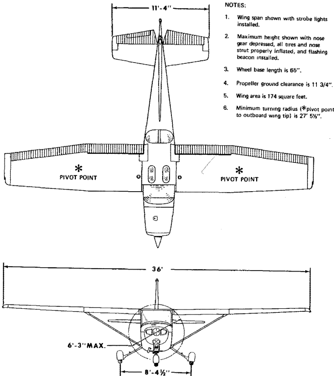
Figure 1-1. Three View
