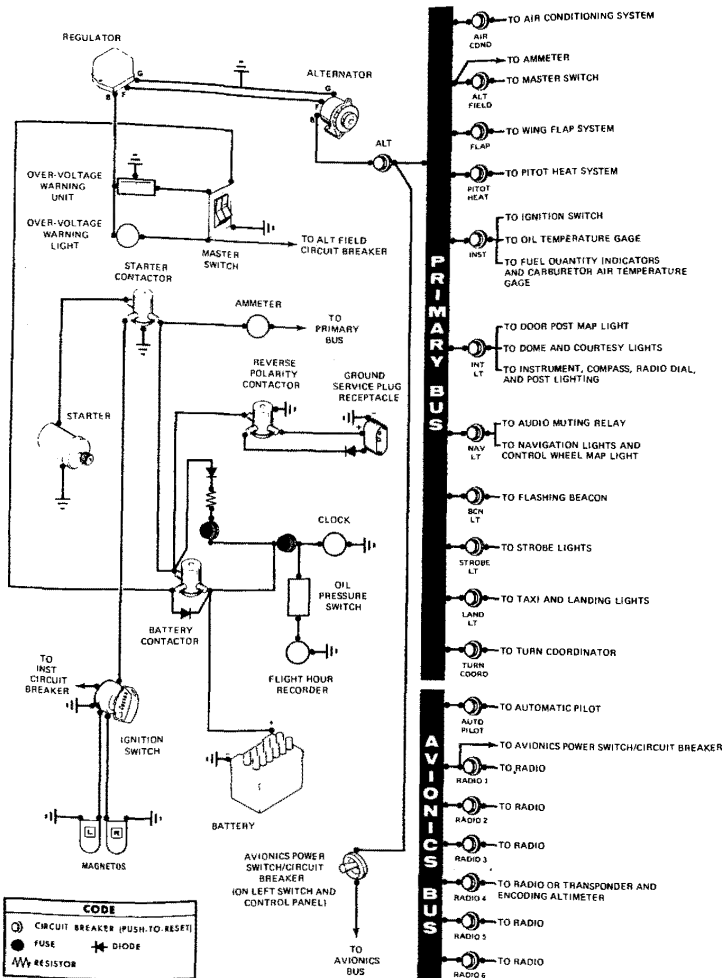
Figure 7-7. Electrical System
