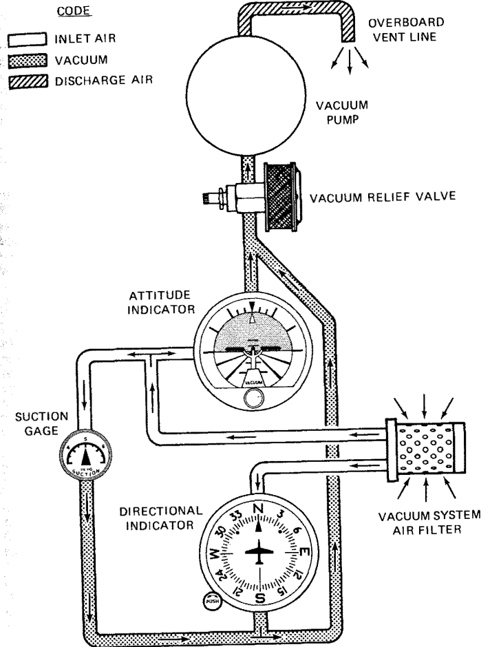
Figure 7-9. Vacuum System
