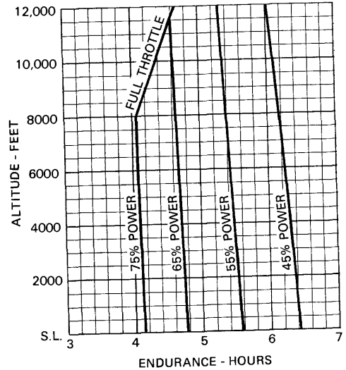
Figure 5-9. Endurance Profile (Sheet 1 of 2)
